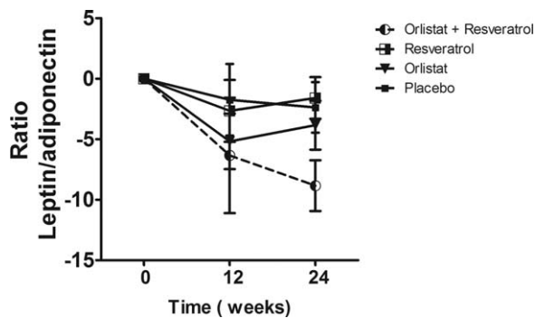
Figure 4 Difference in the leptin/adiponectin ratio decrease whereby participants were randomly assigned to consume placebo, resveratrol, orlistat, or orlistat + resveratrol, as well as an energy-reduced diet, for 24 weeks. Data are presented as the means ± SEM; the statistical analysis was performed using two-way ANOVA to assess the time × treatment interaction ( P < 0.05 ).
