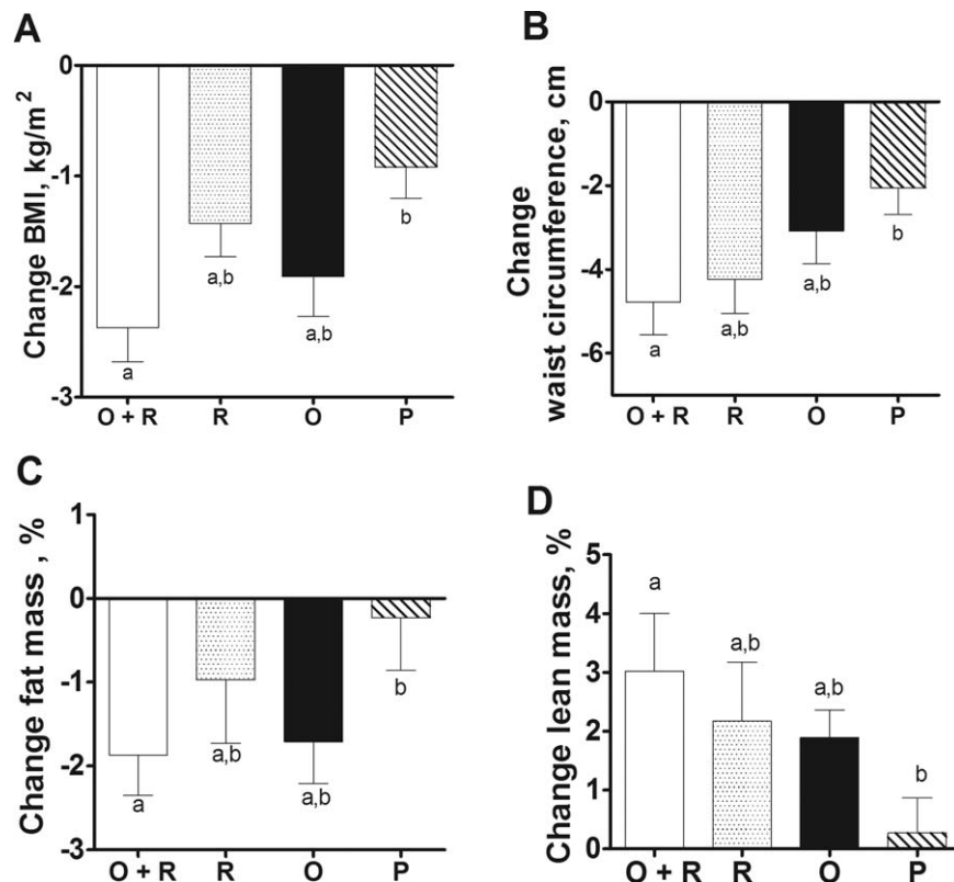
Figure 3 Change in the different anthropometric and clinical parameters after treatment with orlistat + resveratrol (O-R); resveratrol (R); orlistat (O); or placebo (P). (A) Change in BMI with different treatments; (B) change in waist circumference; (C) change in fat mass percentage; (D) change in lean mass percentage. Data are presented as the means \pm SEM; among-group differences were assessed using one-way ANOVA, followed by a multiple comparison by the Bonferroni test, and the differences are shown as different letters in each bar ( a > b > c ).
